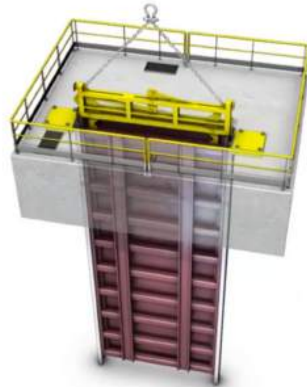
STOP GATES / STOP LOGS
