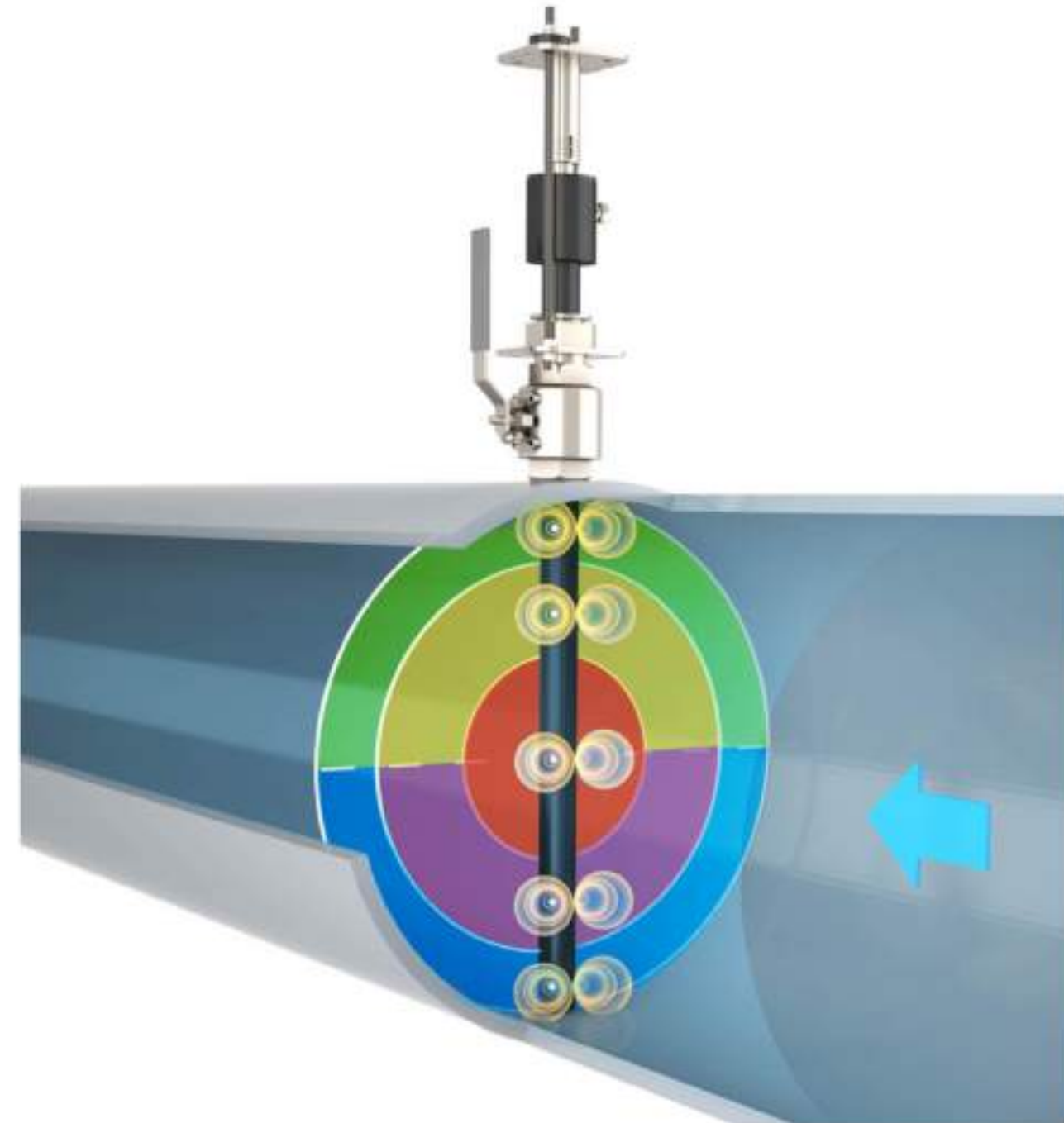
Hot Tap Full Profile Electromagnetic Insertion Flowmeter
