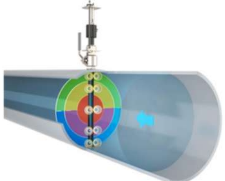
FULL PROFILE ELECTROMAGNETIC INSERTION FLOWMETER
